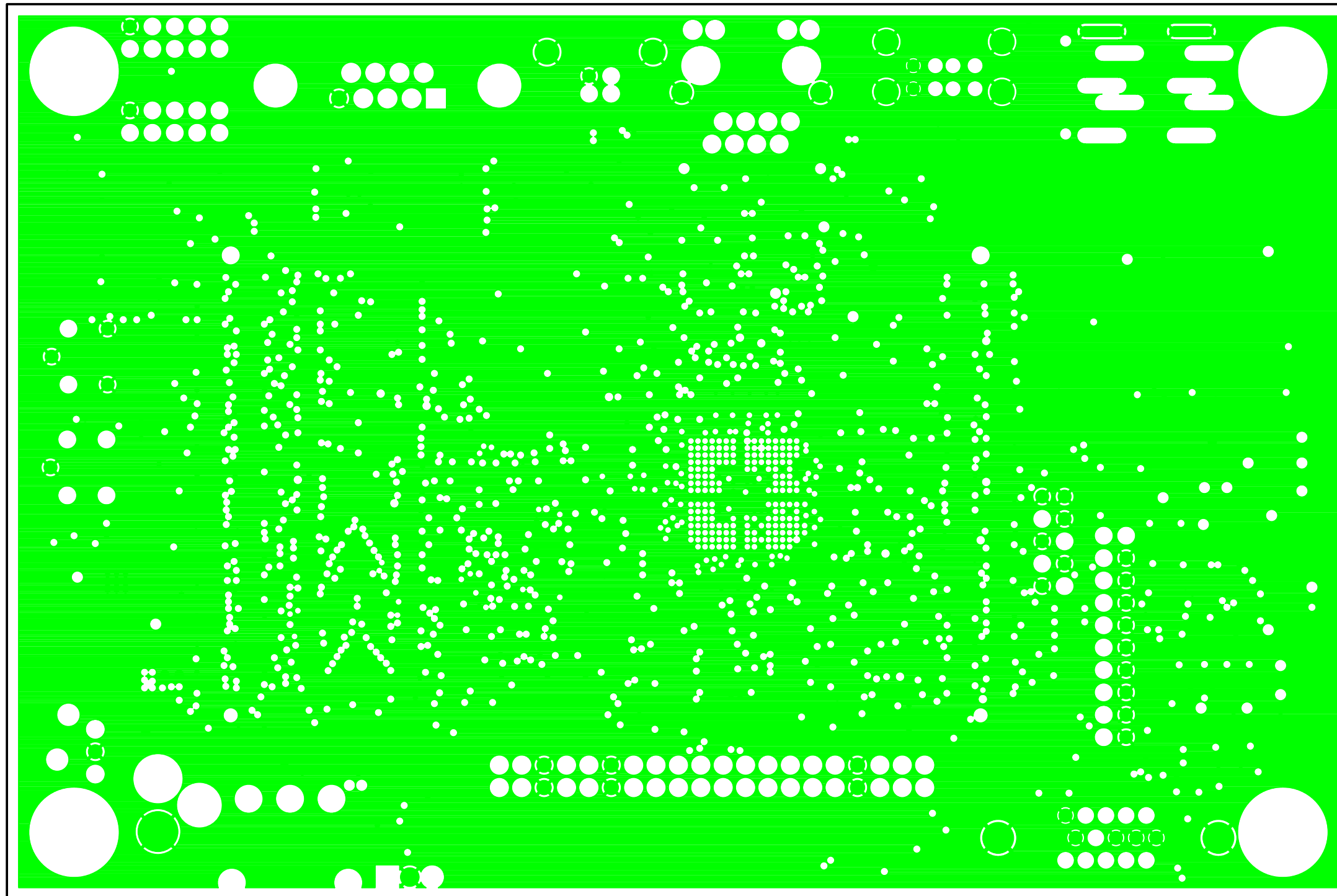
PCB-240-00224-Z1_REV_B LAYER5 GND PLANE
