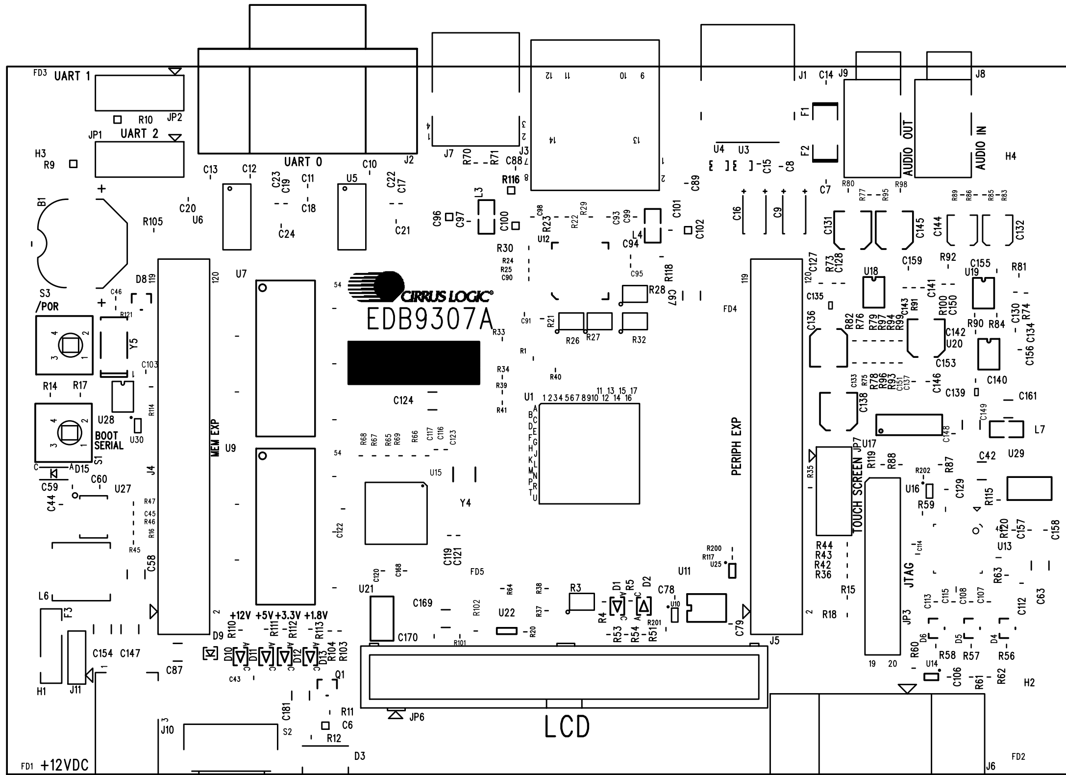
PCB-240-00224-Z1_REV_B SILKSCREEN TOP
